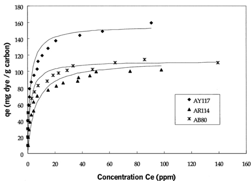
Figure 1. Langmuir isotherm plot for three acid dyes.
