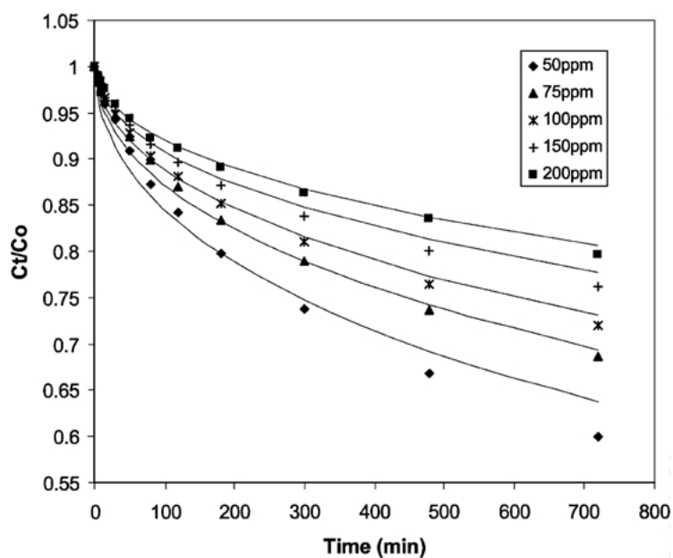
Figure 15. Sorption of AB80 onto activated carbon using film pore surface diffusion model. (12 hours)
