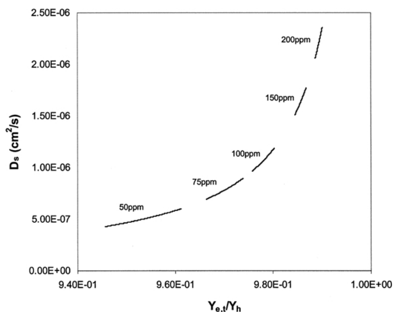
Figure 12. Surface diffusivity against surface coverage. (Acid Yellow 117 System.)
