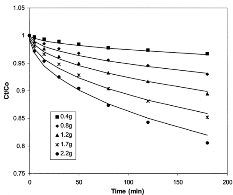
Figure 5. Sorption of AB80 onto activated carbon using film pore surface diffusion model. (Different carbon mass systems.)
