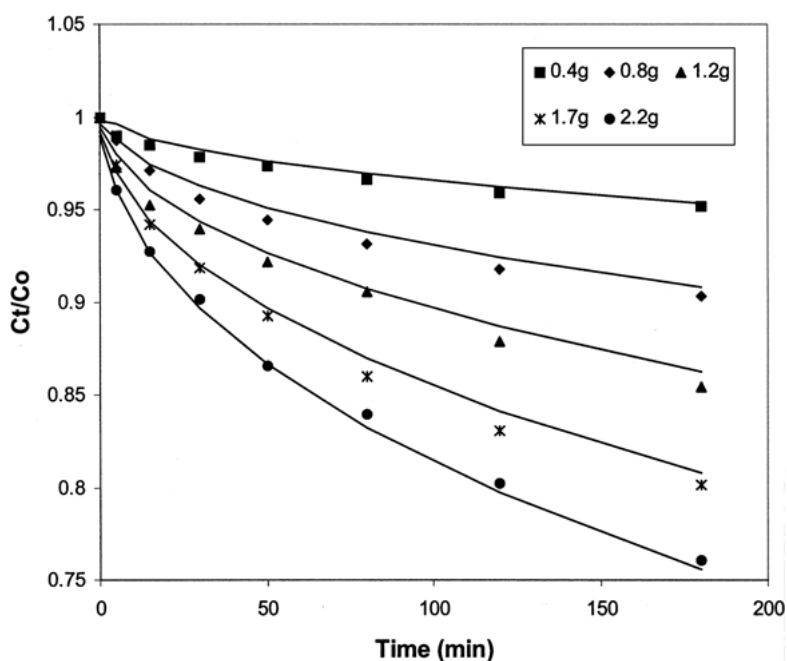
Figure 9. Sorption of AY117 onto activated carbon using film pore surface diffusion model. (Different carbon mass systems.)
