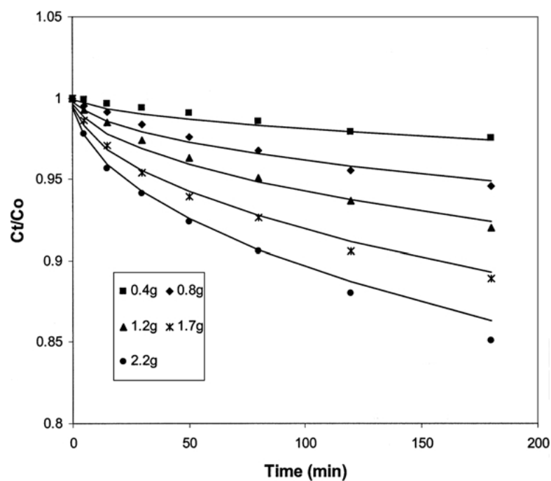
Figure 7. Sorption of AR114 onto activated carbon using film pore surface diffusion model. (Different carbon mass systems.)
