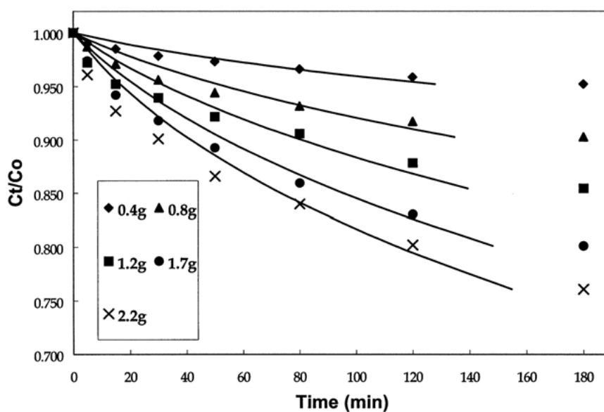
Figure 3. Effect of activated carbon mass on the adsorption of Acid Yellow 117 using the film-pore diffusion model.
